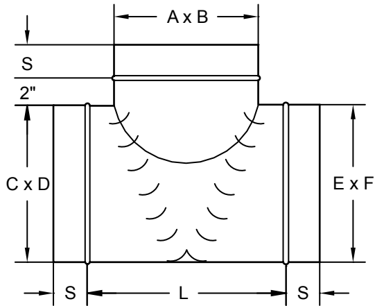
BULLHEAD TEE
