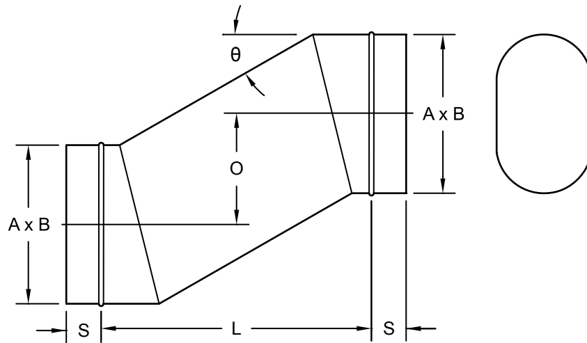
OFFSET HARD
