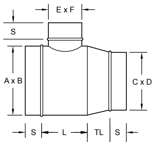
REDUCING TEE
