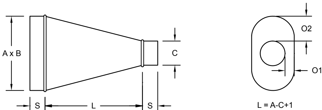
OVAL TO ROUND
