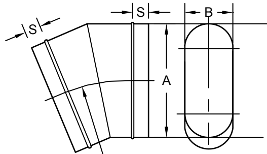
22 \frac{1}{2} ° ANGLE HARD
