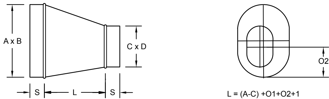
TRANSITION-EASY
