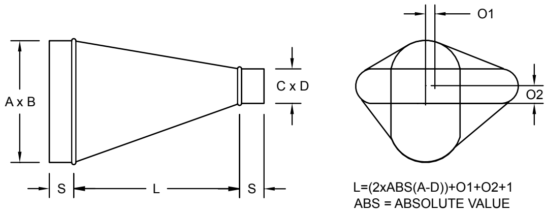
TRANSITION-HARD
