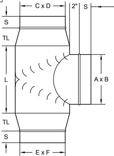
DOUBLE REDUCING BULLHEAD TEE
