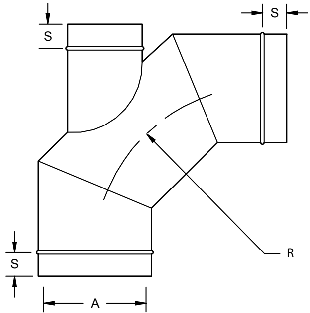
90°HEEL TAP ELBOW (3 PIECE)
