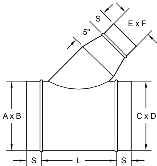
CONICAL LATERAL
