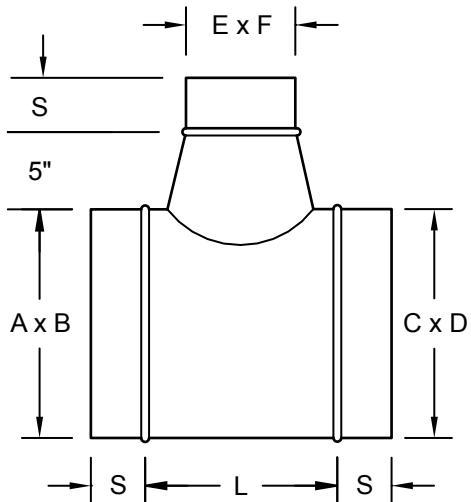
CONICAL TEE
