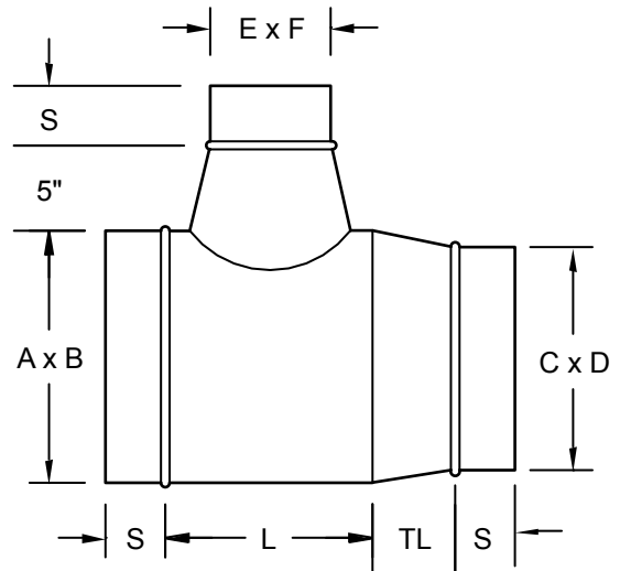
REDUCING CONICAL TEE
