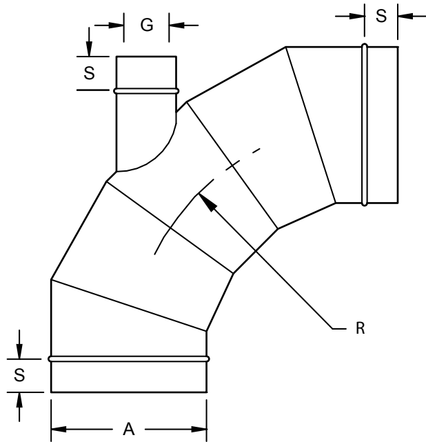
90°HEEL TAP ELBOW (5 PIECE)
