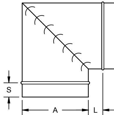
90° MITERED ELBOW (2 PIECE)
