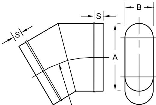
30° ANGLE HARD
