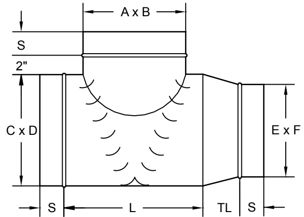
REDUCING BULLHEAD TEE
