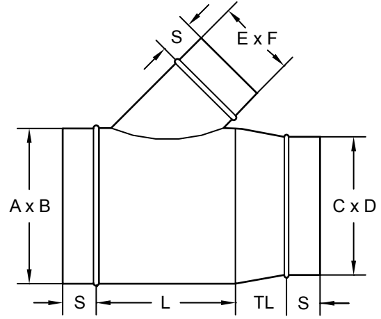
REDUCING LATERAL
