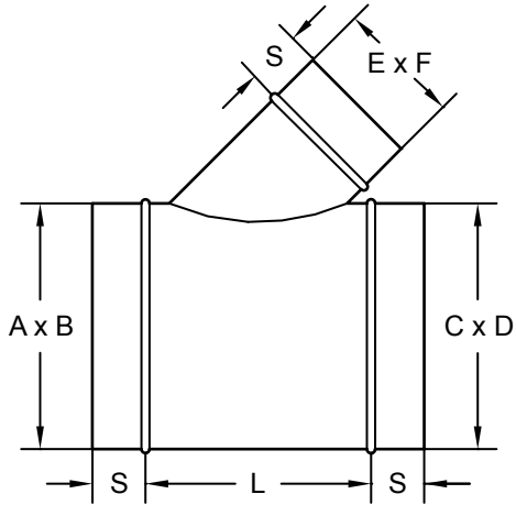
LATERAL
