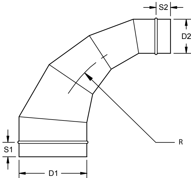
REDUCING 90° ELBOW (5 PIECE)
