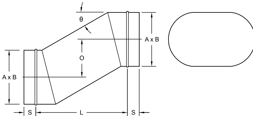
OFFSET EASY
